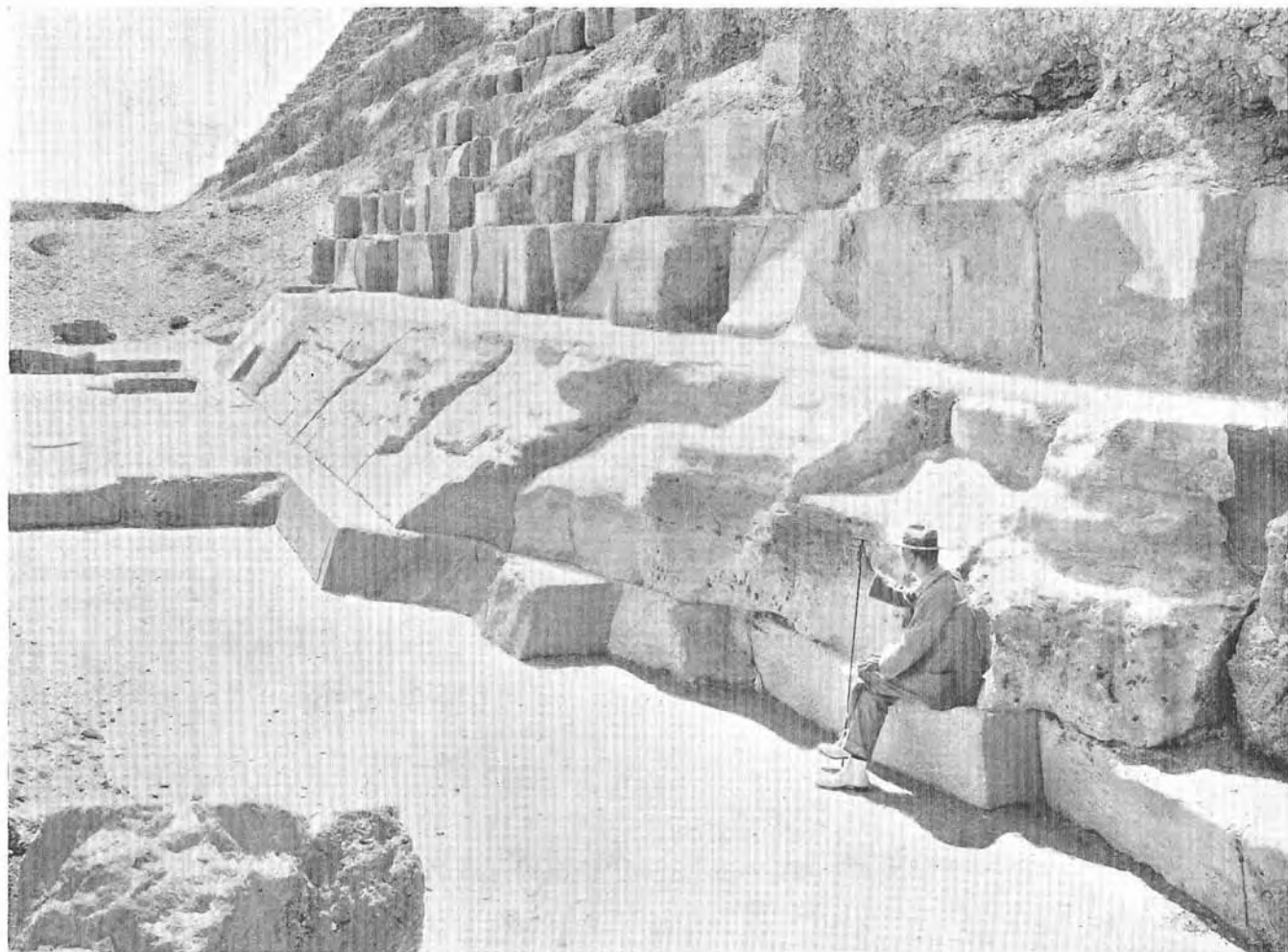
The CASING-STONES of the Great Pyramid of Gizeh (looking east); showing the platform on which they rest, the pavement in front, and the levelled natural rock.
