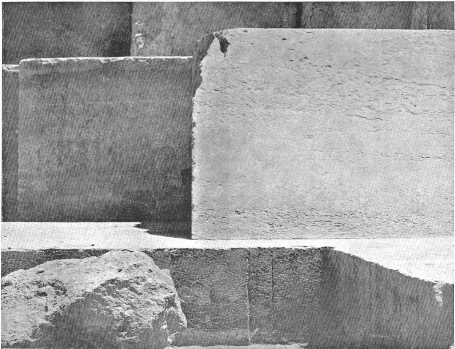
A near front view of the largest of Col. Howard Vyse's historical CASING-STONES of the Great Pyramid of Gizeh; showing the platform on which the casing-stones rest, also a small portion of the pavement to the right, and part of the Pyramid core masonry at the back.
