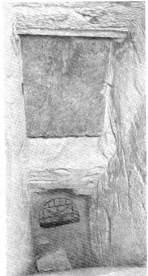
Same as Plate LXVI, but with the debris removed, thus revealing Petrie's granite block on which the iron grill-door is fixed, also Smyth's limestone block which lies end-on against the granite block.
