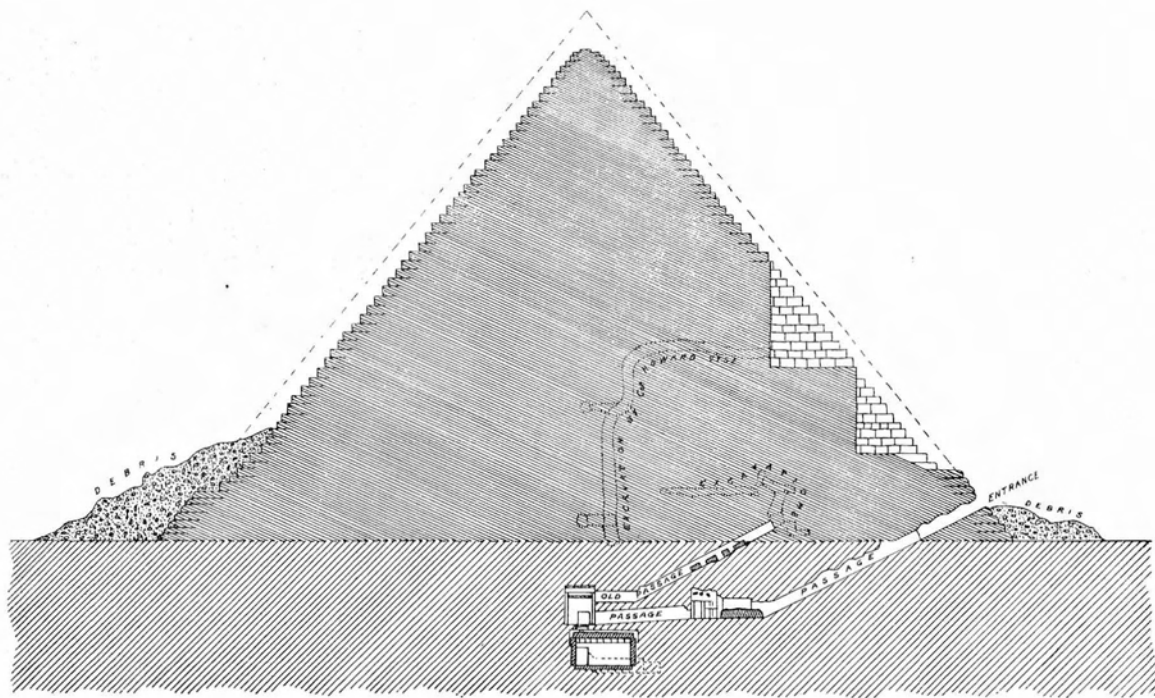
VERTICAL SECTION OF THIRD PYRAMID OF GIZH (FROM NORTH TO SOUTH, LOOKING WEST) SHOWING THE SYSTEM OF ROCK-HEWN PASSAGES AND CHAMBERS AS DISCOVERED BY COL HOWARD VYSE, 1837, A.D.
